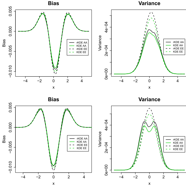
Fig. 1. Plots of the bias (left) and variance (right) of both recursive (rKDE, black) and traditional (KDE, green in color/gray in grayscale) kernel density estimates with sample sizes n = 1000 from Model (i) (top) or Model (ii) (bottom). The form of density estimators are given by (15) and (24) for recursive and traditional ones. Each result is averaged over 10^4 replications. The solid lines are empirical estimates (EE), while the dashed lines are average asymptotic values (AA) for either bias or variance discussed in Section III-D.
