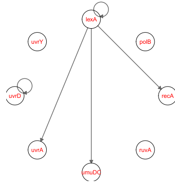
Fig. 5. Reconstruction of SOS DNA repair network by linear VAR model.
