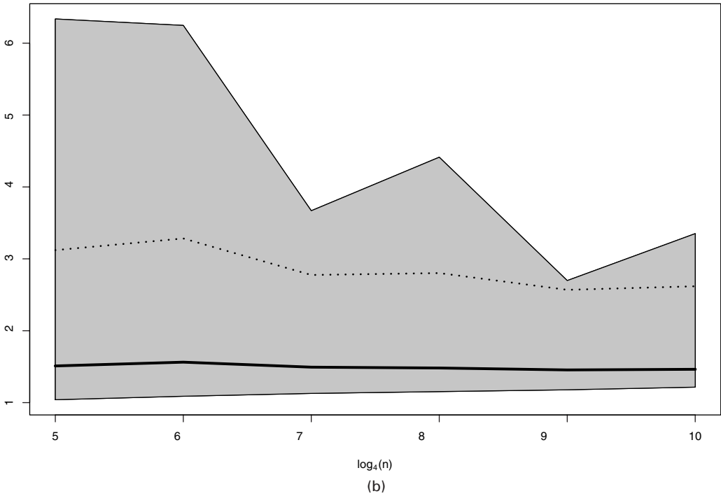
Fig. 2. (a) Contour plot of the density of the logit transform of the \mathcal{N}\{-5, 10, \sigma^2 I_2\} distribution and (b) summary of the successive evaluations of C_\sigma/C_1 = \sigma^2 = 1.5 by averages over the groups \mathcal{G}_n for the logit transform of a single simulated value (x_1, x_2) \sim \mathcal{N}\{-5, 10, \sigma^2 I_2\} : —, average over 100 replications; ■, range of the evaluations; ·····, 2-standard-deviations upper bound
