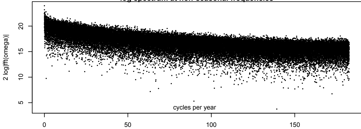
log averaged non-seasonal spectrum
