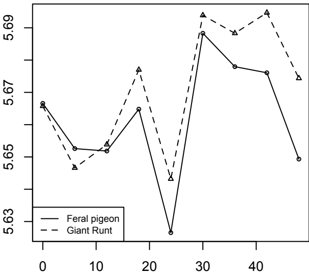
Log metathorax width versus time
