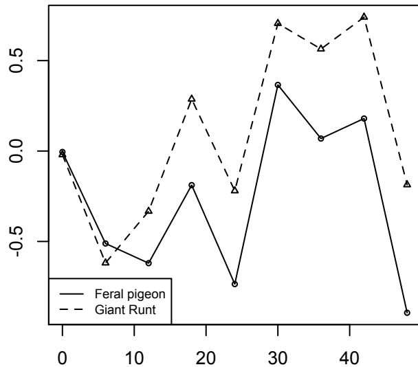
PC1 versus time
