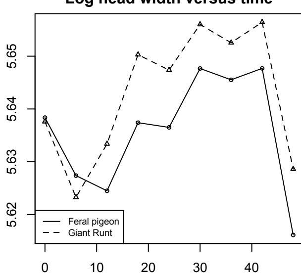
Log head width versus time
