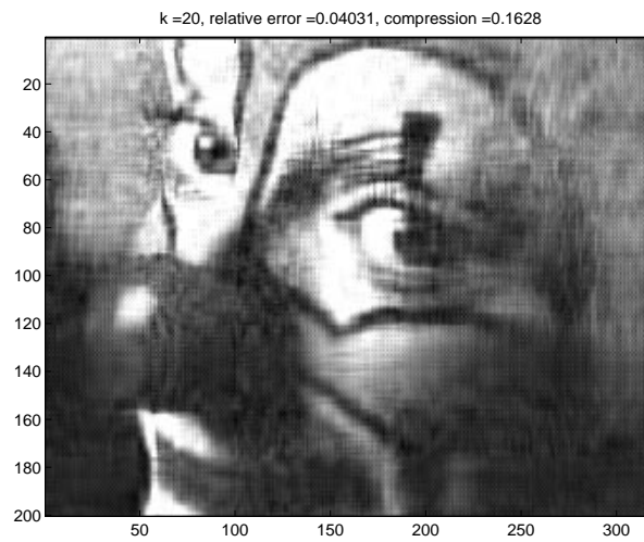
Fig. 3.3. Continued. (c) Rank k = 10 approximation. (d) Rank k = 20 approximation.
