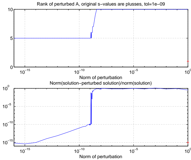
Fig. 3.4. Graph of truncated least squares solution of \min_{y_1} \|(A_1 + \delta A)y_1 - b_1\|_2 , using \text{tol} = 10^{-9} . The singular values of A_1 are shown as red pluses. The norm \|\delta A\|_2 is the horizontal axis. The top graph plots the rank of A_1 + \delta A , i.e., the numbers of singular values exceeding \text{tol} . The bottom graph plots \|y_1 - x_1\|_1 / \|x_1\|_2 , where x_1 is the solution with \delta A = 0 .
