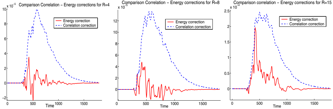
FIG. 5.5. Comparison correlation correction - energy correction, for 8% fluctuations, for the radii R = 4 , R = 8 and R = 15 , respectively. The case R = 15 is averaged over 2 realizations while the cases R = 8 and R = 4 are averaged over 4 realizations.
