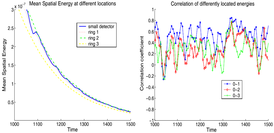
FIG. 5.4. Left: Averaged energies over D_0 and the rings G_k , k = 1, 2, 3 . Right: Correlations C_{0k} for k = 1, 2, 3 .
