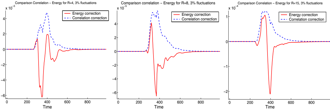
FIG. 5.6. Comparison correlation correction - energy correction, for 3% fluctuations, for radii equal to R = 4 , R = 8 and R = 15 . The ballistic part of the waves is significant.
