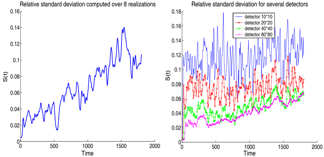
FIG. 5.3. Left: S(t) performed over 8 realizations, for a 40 \times 60 detector located at the center of the domain. Right: S(t) performed over 20 realizations and computed for 4 different detectors located at the center.
