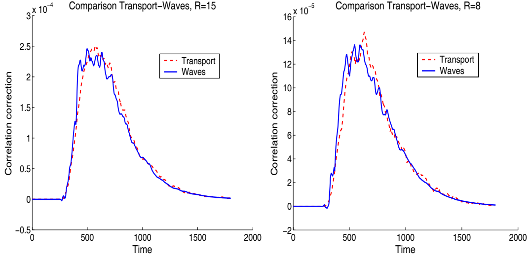
FIG. 5.2. Verification of the accuracy of the modified transport regime: comparison wave in changing media - transport equations, for 8% fluctuations. We plot \delta\mathcal{E}_{cor} and \delta\mathcal{A}_{cor} . The domain of computation is that of fig. 5.1. The R = 15 (resp. R = 8 ) case on the left (resp. right) is averaged over 2 (resp. 4) realizations.
