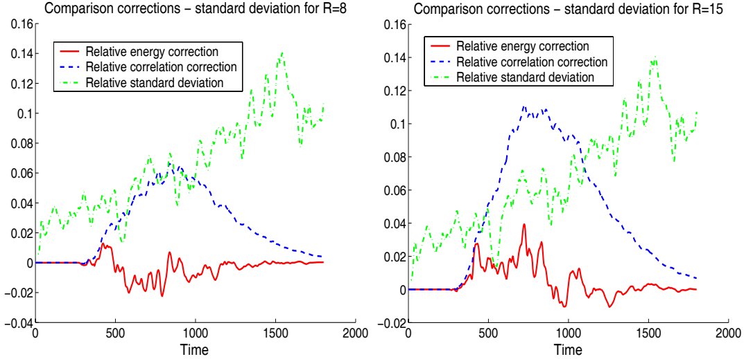
FIG. 5.7. Comparison relative standard deviation - relative correlation correction - relative energy correction, for 8% fluctuations and R = 8 (left) and R = 15 (right).
