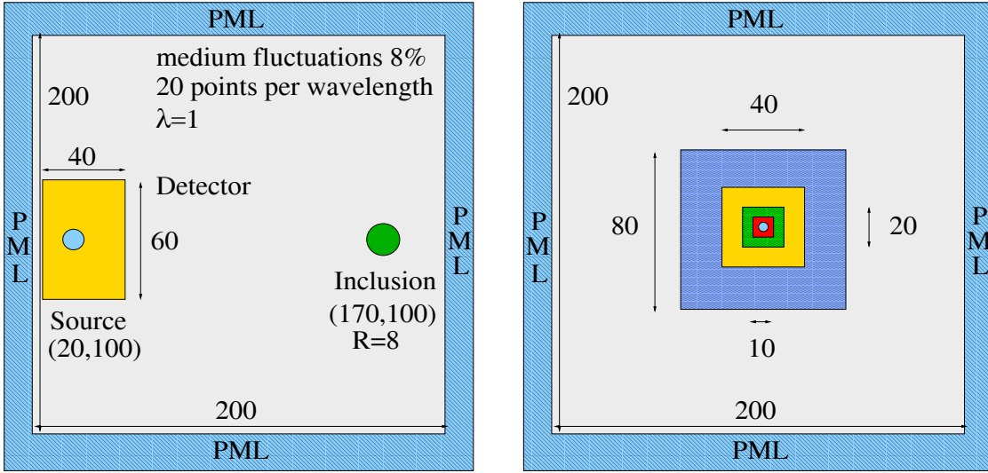
FIG. 5.1. Domains of computation used in the numerical experiments.
